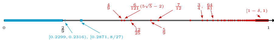
Figure 1: Current partial picture for jumps and non-jumps of 3-graphs.
